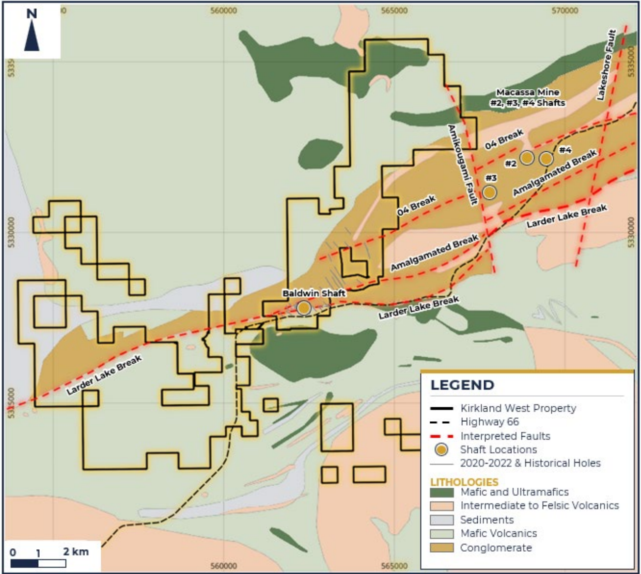
Figure 3: Map showing simplified main lithologies and structures Kirkland Lake West
