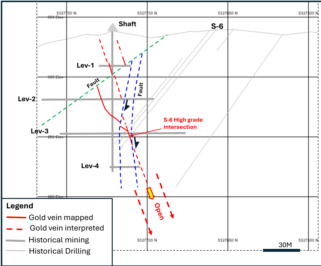
Figure 4: Simplified schematic vertical section looking NE showing historical Hole 6, the Baldwin shaft, and underground development on four levels *
